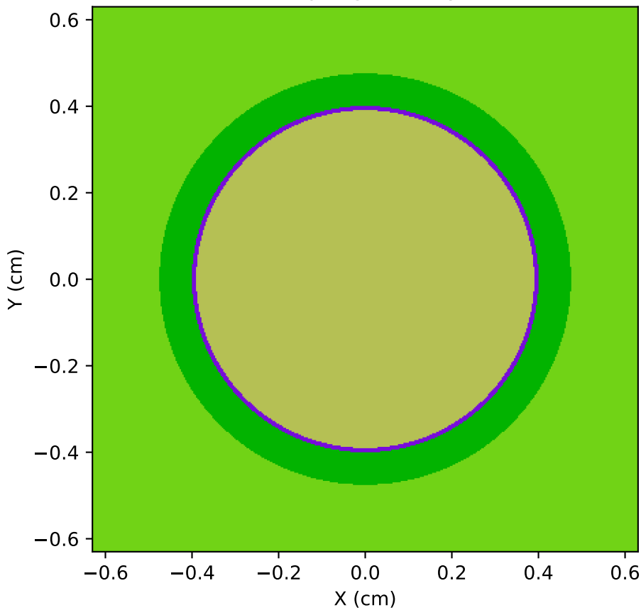
2D pin geometry
